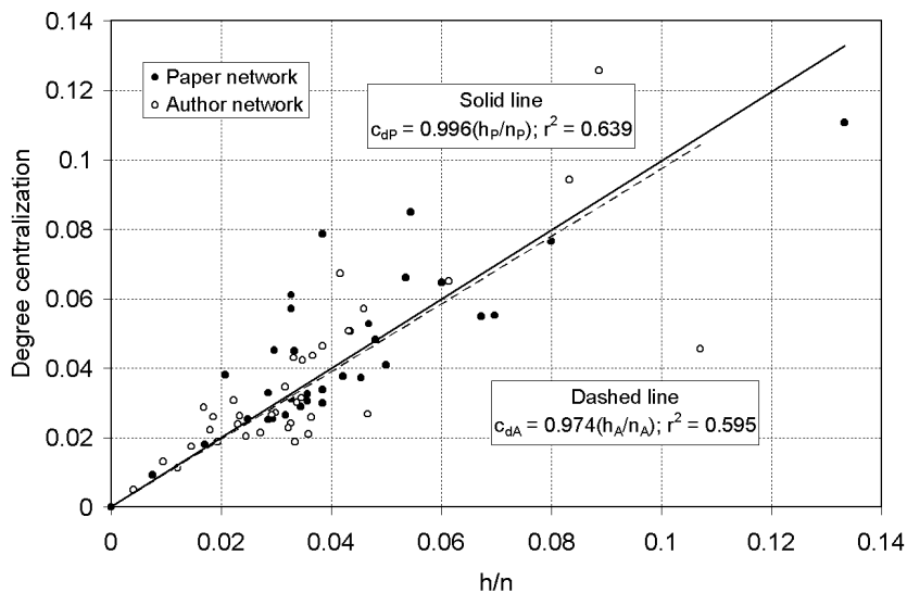
Figure 2. Correlation of degree centralization with the degree h-indices
