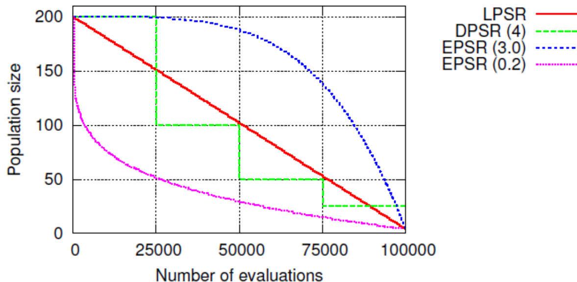
Comparison of reduction strategies
