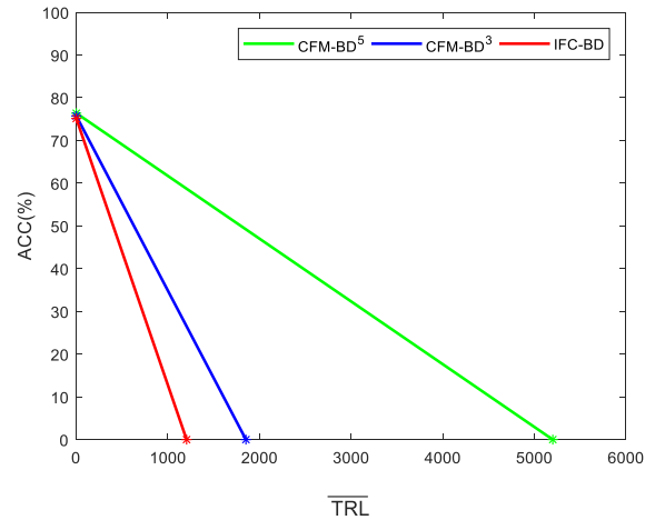
Fig. 3. Models' tradeoff: \overline{\text{TRL}} versus ACC.
