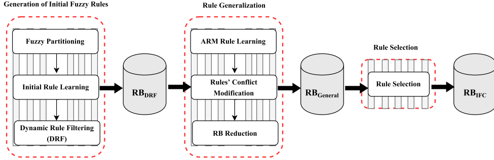
Fig. 1. General schema of IFC-BD: An illustration of the RB evolution.
