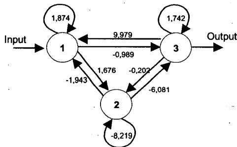
FIG. 2: RANN THAT EMULATE THE MACKEY-GLASS FUNCTION
