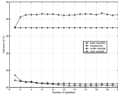
Fig. 3. Test error for different number of base classifiers.
