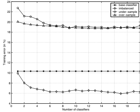
Fig. 2. Training error for different number of base classifiers.
