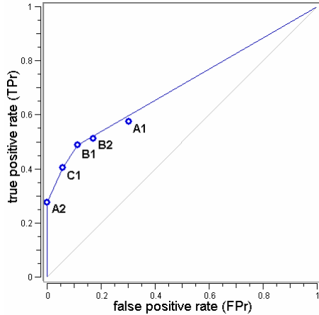
Figure 4: Representation of subgroups in ROC space.
