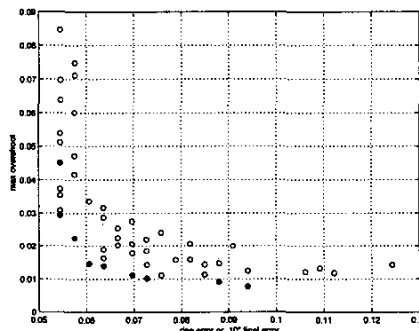
Figure 3: Non-dominated optimisation surface
