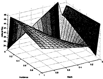
Figure 4: Control surface for \omega_n
