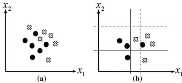
Fig. 3 Two-class classification problems with bidimensional patterns. When missing values occur, they are represented by a vertical or horizontal line, depending on which attribute is unknown
