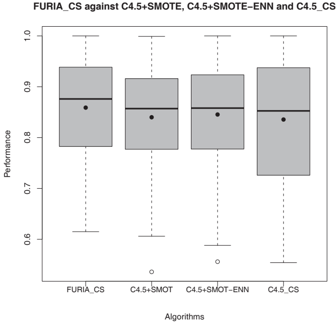
Fig. 2. Performance of FURIA_CS and C4.5 with preprocessing approaches and cost-sensitive learning.
