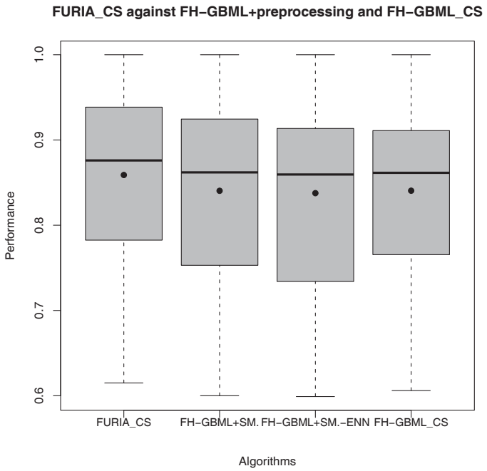
Fig. 5. Performance of FURIA_CS and FH-GBML with preprocessing approaches and cost-sensitive learning.
