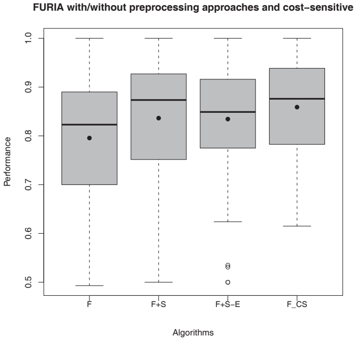
Fig. 1. Dispersion of the performances of FURIA, FURIA+SMOTE, FURIA+SMOTE+ENN and FURIA_CS.
