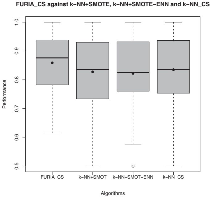
Fig. 4. Performance of FURIA_CS and k-NN with preprocessing approaches and cost-sensitive learning.
