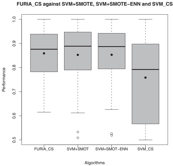
Fig. 3. Performance of FURIA_CS and SVM with preprocessing approaches and cost-sensitive learning.
