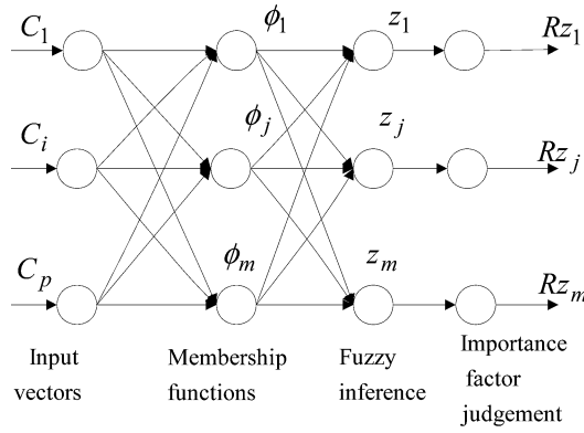
Fig. 2. Neural fuzzy model for feature selection.
