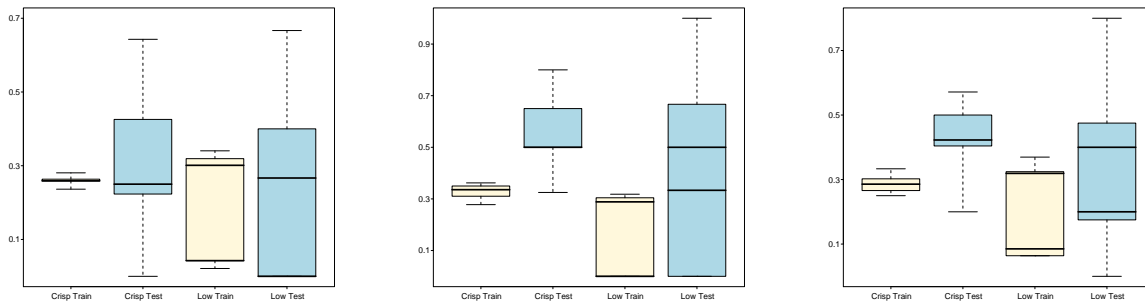
Fig. 15 Boxplots illustrating the classification error of crisp and extended GFS in the high performance athletics problem. From left to right: Problems “100ml-4-I”, “Long-4”, and “100ml-4-P”.
