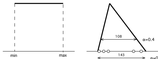
Fig. 1 Fuzzy representation of vague data. Left: A missing value is codified with an interval that spans the whole range of the variable, or P([\min, \max]) \leq 1 . Right: A compound value (in this example, five different measurements of the variable) can be described by a fuzzy membership, that can also be understood as an upper probability. Each \alpha -cut contains the true value of the variable with probability at least 1 - \alpha .
