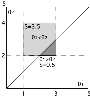
Fig. 8 Graphical representation of the example 1, showing that [1, 3] \prec [2, 4] .
