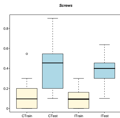
Fig. 11 Boxplots illustrating the error of crisp (columns ‘CTrain’ and ‘CTest’) and extended GFS (columns ‘ITrain’ and ‘ITest’) in the problem “Screws”.
