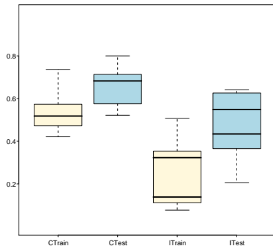
Fig. 13 Boxplots illustrating the results of crisp (columns ‘CTrain’ and ‘CTest’) and extended GFS (columns ‘ITrain’ and ‘ITest’) in the problem “dyslexia-12”, with 4 labels/partition.
