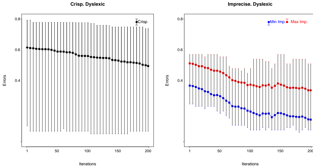
Fig. 14 Compared evolution of crisp (left) and imprecise GFS (right) in the dataset “dyslexia-12”. The minimum, mean and maximum classification error at every generation are shown, for both the crisp and the imprecise versions of the algorithm. The upper bound of the imprecise fitness is consistently lower than the crisp fitness.
