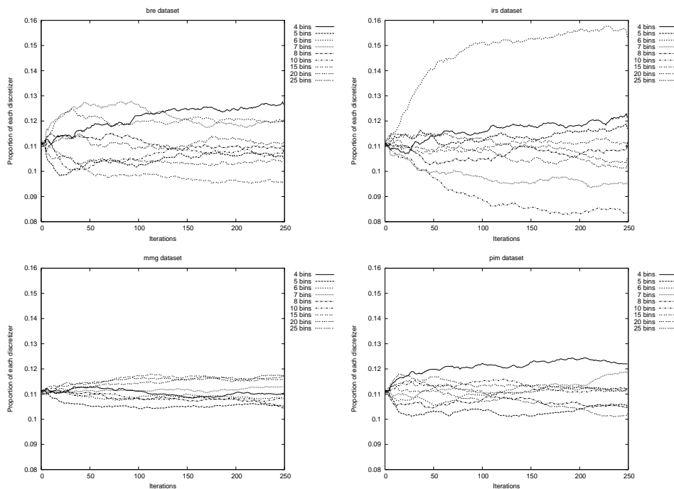
Fig. 2. Evolution of the discretizer proportions in the population for the bre , iris , mmg , pim datasets
