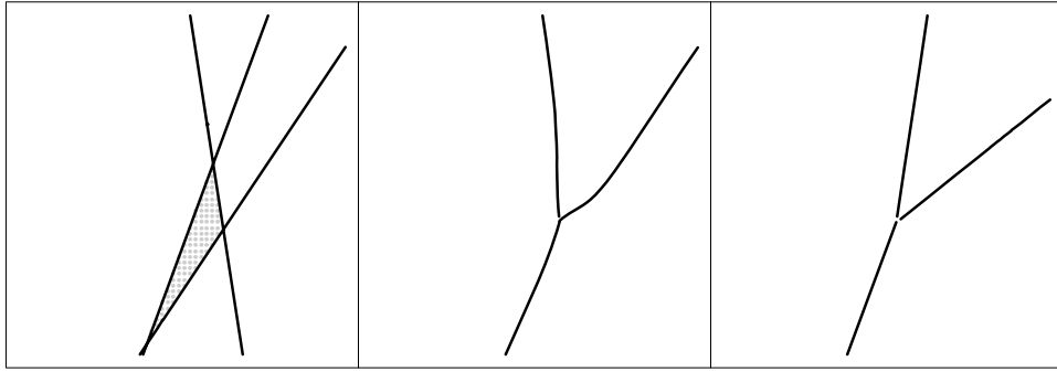
Figure 1: A three class problem, with the data in each class generated from a mixture of Gaussians. The first panel shows the maximum-win procedure. The second panel shows the decision boundary from coupling of the pairwise linear discriminant rules based on \hat{d} in (6). The third panel shows the three-class LDA boundaries. Test-error rates are shown in parentheses.
