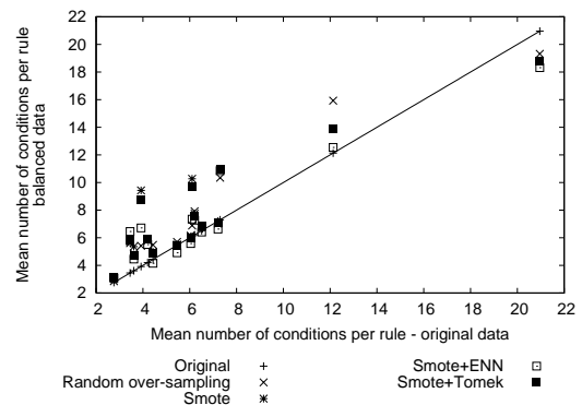
Figure 7: Mean number of conditions per rule for original and balanced data sets and unpruned decision trees.
